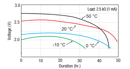
Discharge temperature characteristics (Example: BR435)
