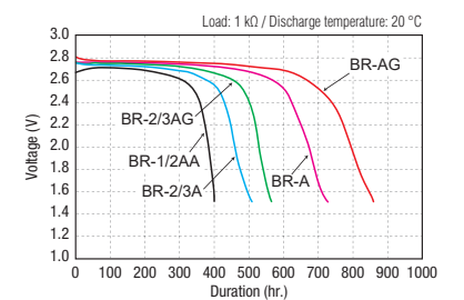
Example discharge characteristics
