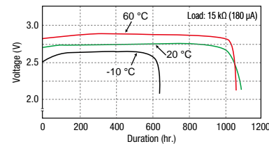
■ Discharge temperature characteristics (Example: BR2032)
