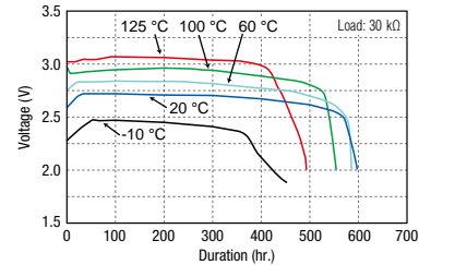
■ Discharge temperature characteristics (Example: BR1225A)
