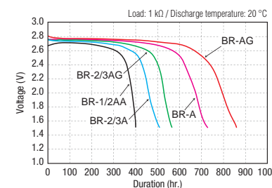
Example discharge characteristics
