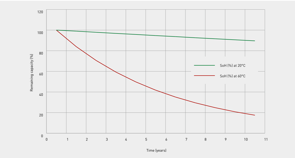
VL/ML CAPACITY DEGRADATION UNDER FLOAT
