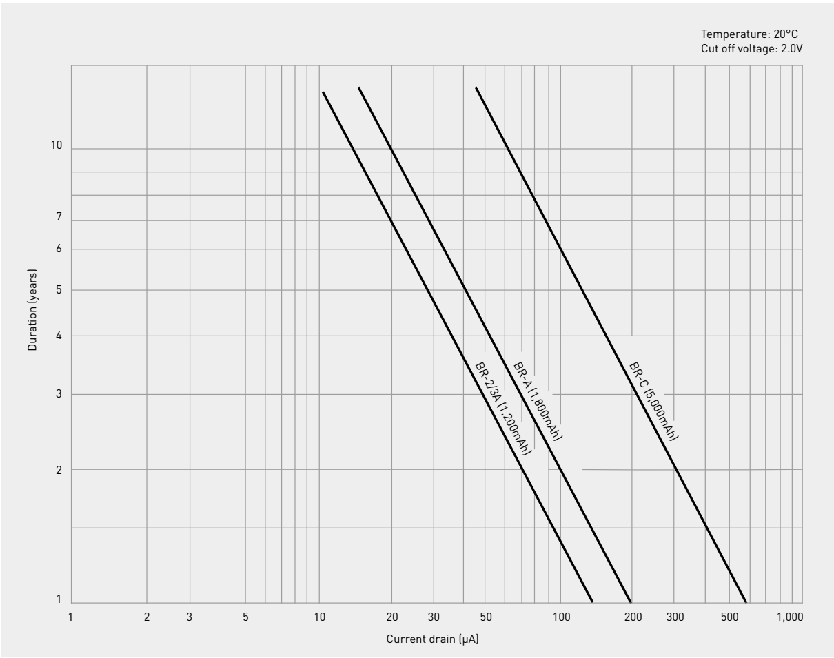
GENERAL FORMULA (ROUGH VALUE WITH 20°C, STANDARD LOAD)
