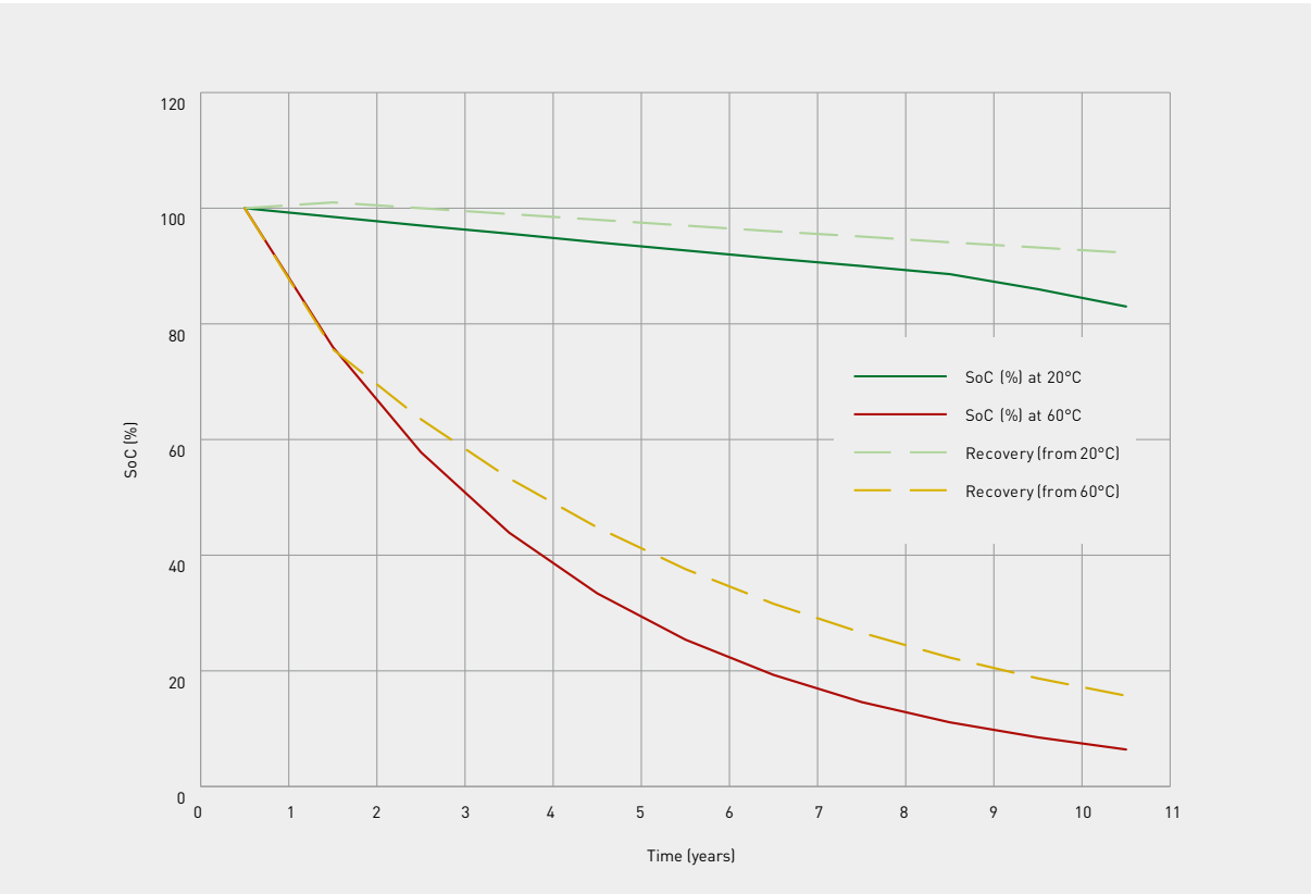
VL/ML CAPACITY DEGRADATION UNDER FLOAT
