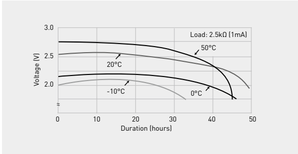
OPERATING VOLTAGE VS. DISCHARGE CURRENT**
